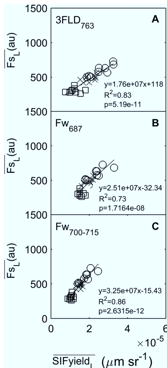
Fig. 3. Leaf-average scale relationship between active (F sL ) and passive (SIFyield L ) measurement, using (A) F s700–715 and 3FLD 763 techniques, (B) F s700–715 and Fw 687 techniques, and (C) F s700–715 and Fw 700–715 techniques in wheat plants under low (square), medium (cross) and high (circle) fertilization treatment. Each point represents the leaf replicates fluorescence mean ( n=9 ) per day (days=9). The black line represents a regression between active and passive techniques ( P<0.01 ).
