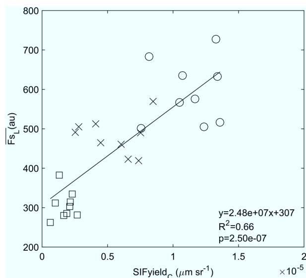
Fig. 2. Canopy and leaf-average scale relationship between active leaf-average (F sL ) and passive canopy (SIFyield C ) measurements using F s700–715 and 3FLD 763 techniques in wheat plants under low (square), medium (cross) and high fertilization treatment (circle). For leaf level measurements, each point represents the leaf replicates fluorescence mean ( n=9 ) per day (days=9). The black line represents a regression between active and passive techniques ( P<0.01 ).
